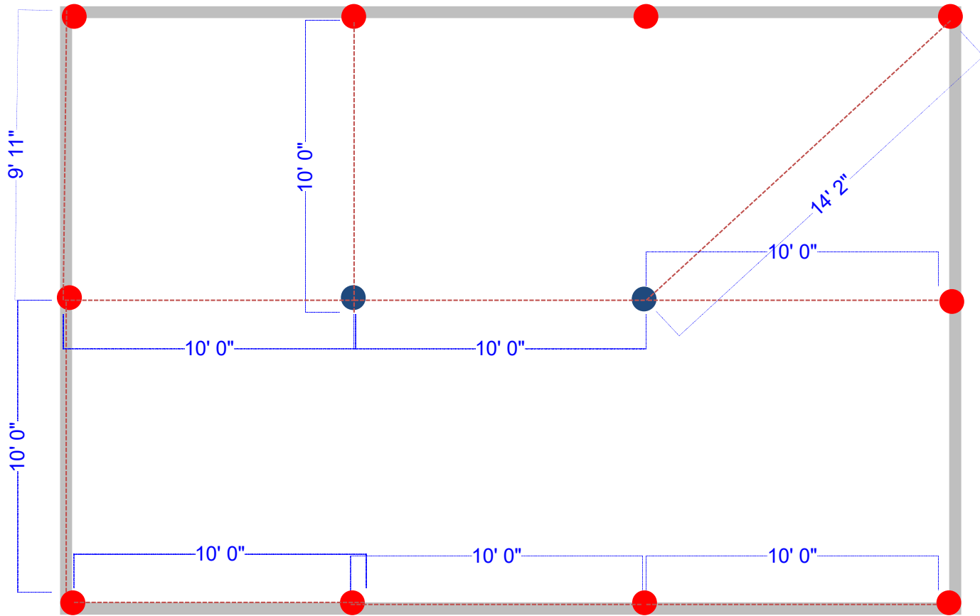
20' x 30' pole Tent - Pole placement
